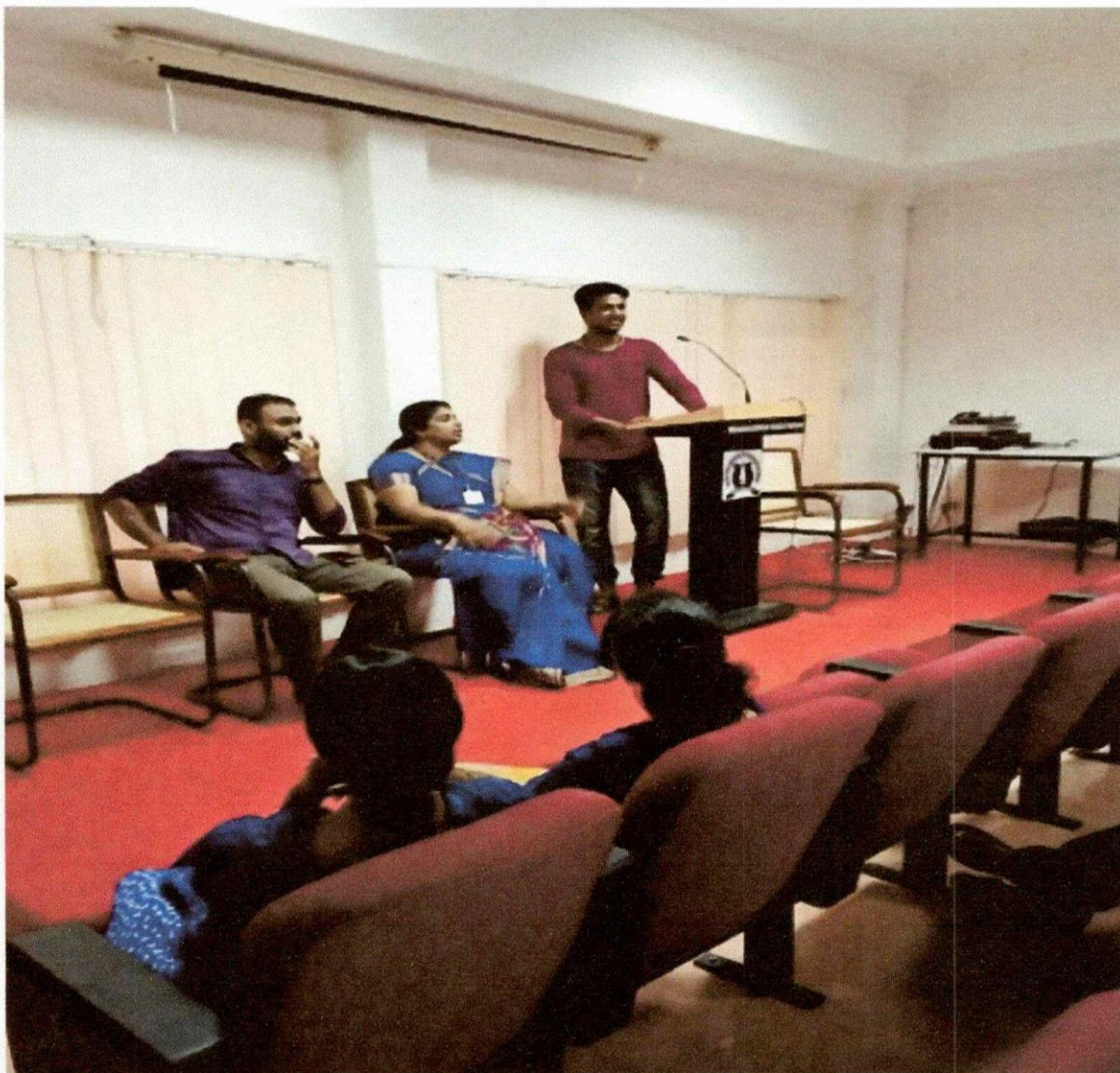
Orientation Class
